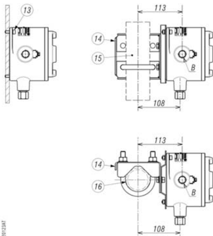
Fig. 18 – Example of mounting Series BW and BA
