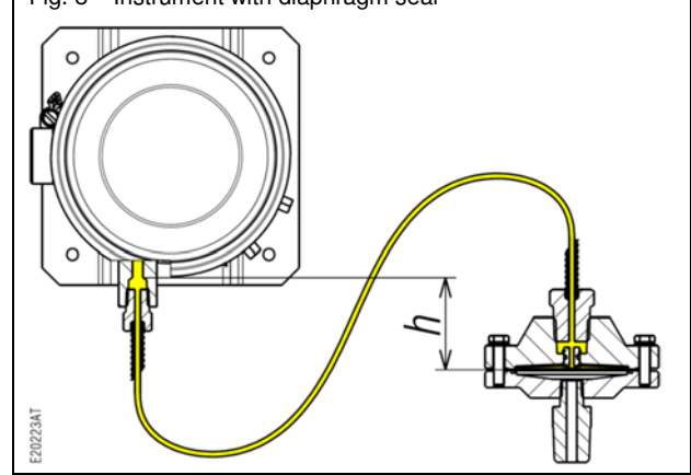
Fig. 8 – Instrument with diaphragm seal
